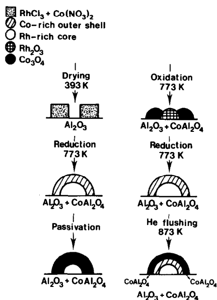
FIG. 6. Formation of bimetallic \text{CoRh} particles during reduction of the impregnated catalyst and the change in structure of the particles after different treatments.
