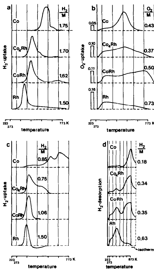
FIG. 4. TPR, TPO, and TPD profiles for alumina-supported Co (4.44 wt%), \text{Co}_4\text{Rh} (4.57 wt%), \text{CoRh} (5.40 wt%), and Rh (2.30 wt%) catalysts. (a) TPR of the impregnated and dried catalysts, (b) TPO of the reduced catalysts, (c) TPR of the oxidized catalysts, (d) TPD of the reduced catalysts, the metal particles of which are covered with hydrogen.
