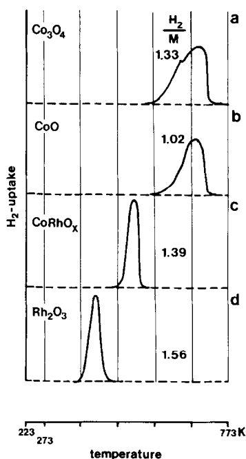
FIG. 3. TPR profiles for bulk oxides. (a) Co 3 O 4 , (b) CoO, (c) CoRhO x , and (d) Rh 2 O 3 .
