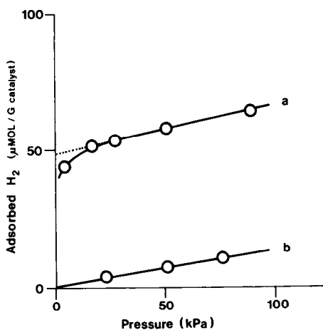
FIG. 1. Hydrogen chemisorption isotherms measured at 298 K for the 0.57 wt% Rh/Al 2 O 3 catalyst. (a) Catalyst, (b) bare support.
